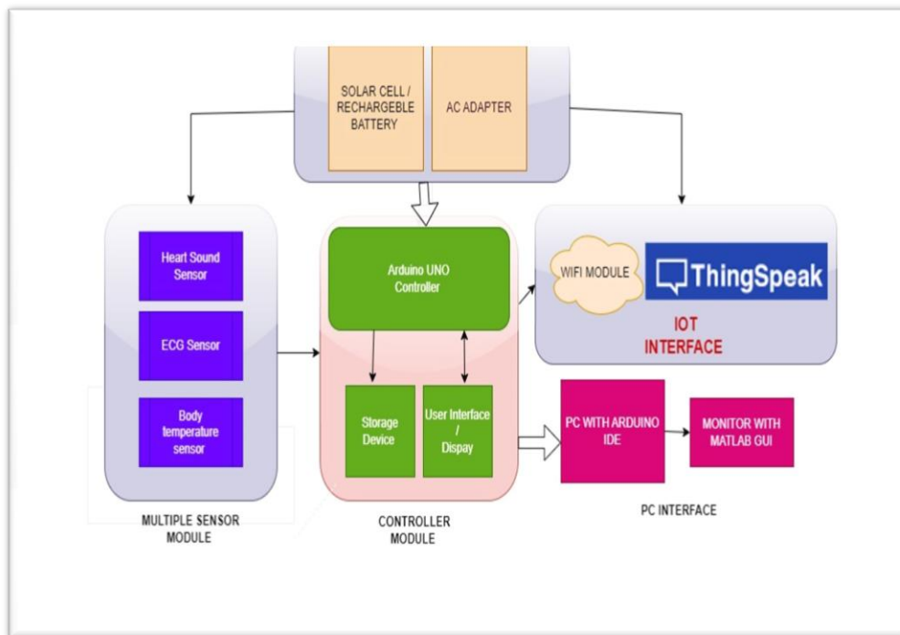
Fig. 1 discloses the overall block diagram of the vital data acquisition system.
